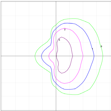
D1 T4 Distance is in Units of Mounting Height Mounting Height 35'
