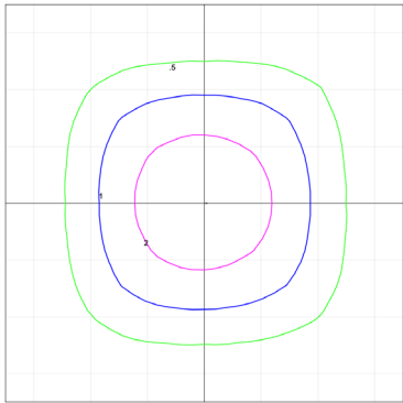
D1 T5 Distance is in Units of Mounting Height Mounting Height 35'
