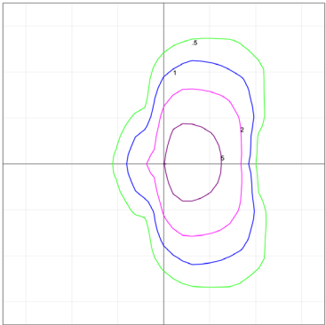
D1 T3 Distance is in Units of Mounting Height Mounting Height 35'
