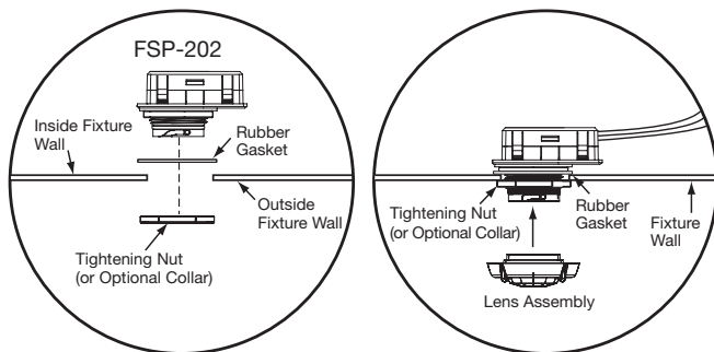
Figure 1. Installing the FSP-202 in the light fixture
